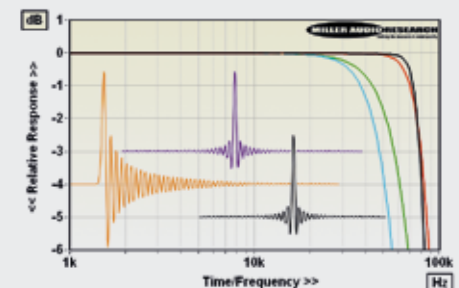
ABOVE: Frequency/impulse Filter responses [Filter 1, black; 2, red; 3, cyan; 4, green; 5, orange; 6, purple]
